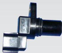
Pulse Generator T41438 Input with OEM Compatible plug, fits F4A42/F4A51/F5A51
