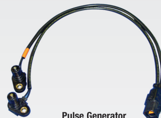
Pulse Generator T42436M Input/Output on Harness with OEM Compatible plug, fits F4A43
