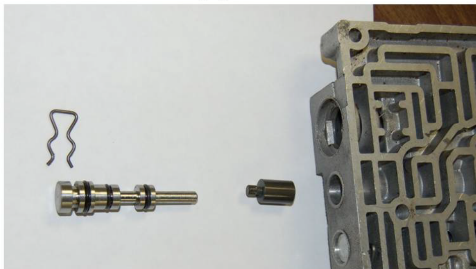
Parts needed for installation of the A74741Q Valve
